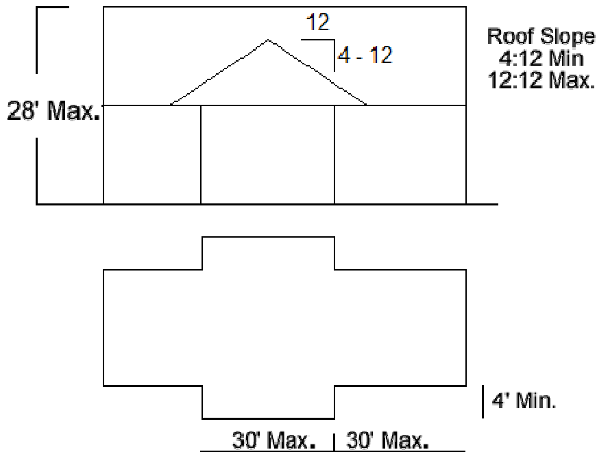
Figure D - Roof Pitch and Massing
